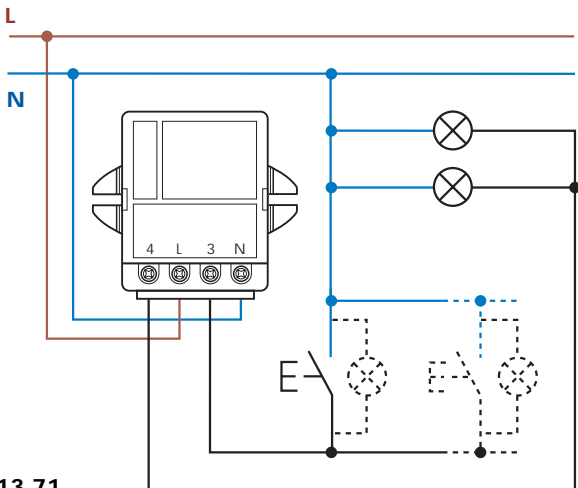
Type 13.71 3 wire connection Max 15 ( \leq 1 mA) illuminated push buttons
