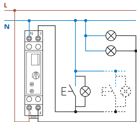
4 wire connection
