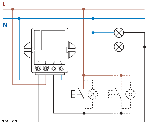
Type 13.71 4 wire connection Max 15 ( \leq 1 mA) illuminated push buttons
