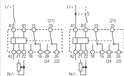
wiring diagram (without signal START)
