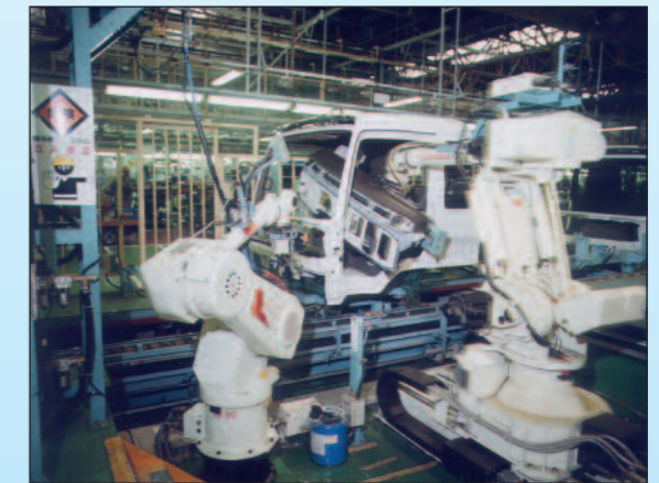
Assembling Montage
