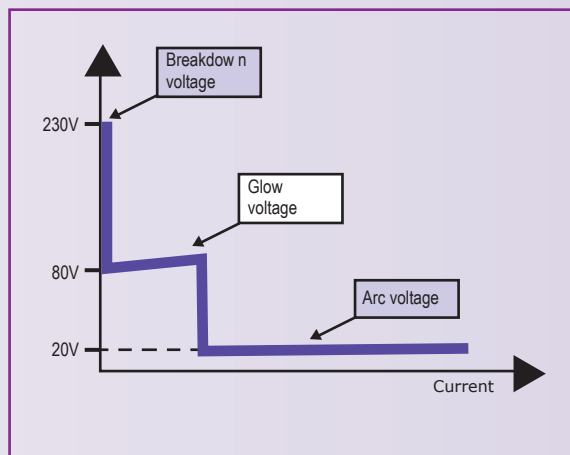
Operating curve
