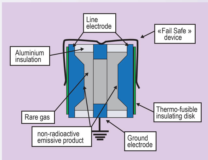
3-electrode gas tube description
