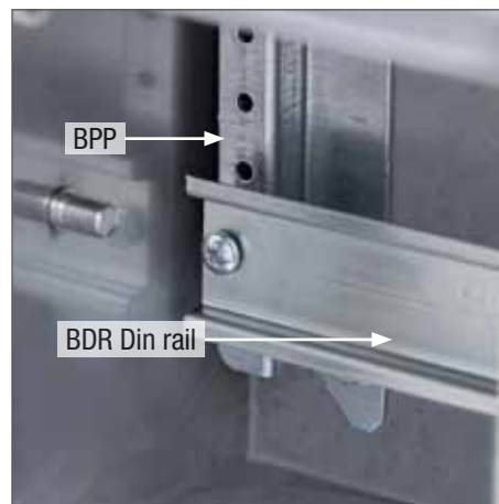
Detail of BPP mounted in “height” flush to the sides
