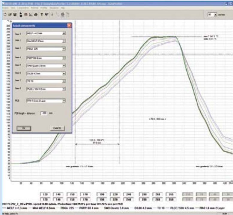
Ersa AutoProfiler with library Off line profiling saves time and money A "Virtual PCB" is created and sent through the "Virtual Oven" – first run success → 90 %
