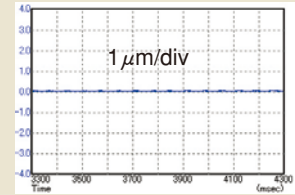
Position deviation at constant speed (Example)
