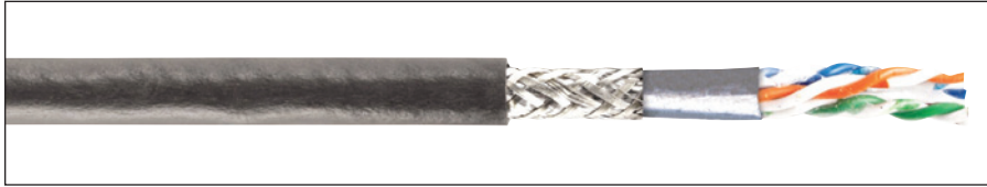
TRANSIT, 4 PAIR/24 AWG, SHIELDED FOIL TWISTED PAIR (SFTP) CAT 5, LOW SMOKE
