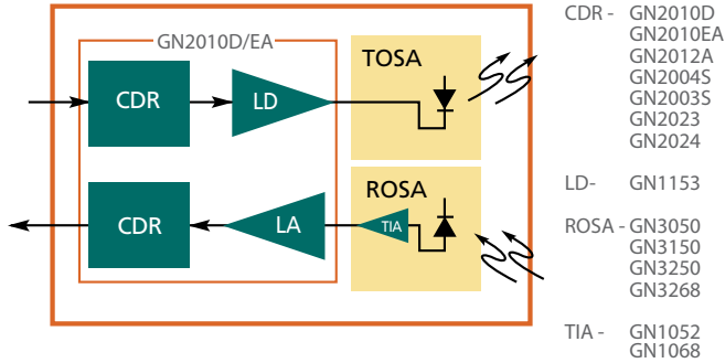
10G XFP Module for \leq 40\text{Km} Applications
