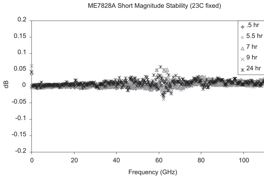
Figure 3. S11 measurement stability of short, ME7828A W1 1mm coaxial test port with MG37022A Fast Switching Synthesizer, over a 24 hour period.
