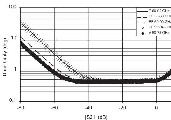
E, Extended-E, and V Band Transmission Phase Uncertainties-LRL
