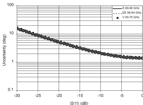
E, Extended-E, and V Band Reflection Phase Uncertainties-LRL
