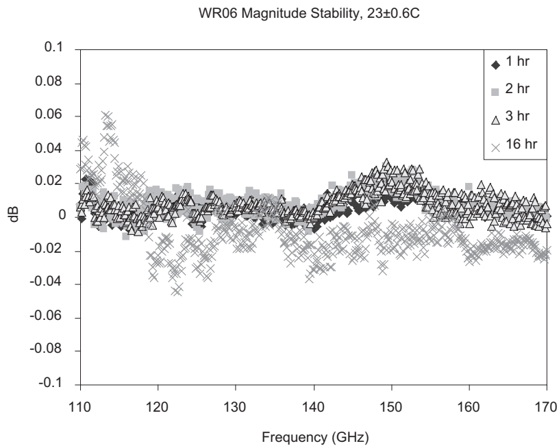
Figure 4. Magnitude stability plot of WR06 110 to 170 GHz using the Wildfire MG37022A fast switching synthesizer as the RF and LO source.
