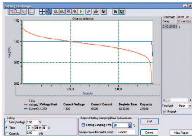
Example of battery discharge characteristics of an AA alkaline battery
