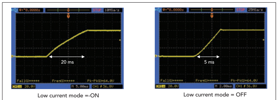
Figure 3: Voltage rise time with and without Low current mode enabled
