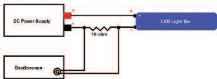
Figure 1 - Setup
