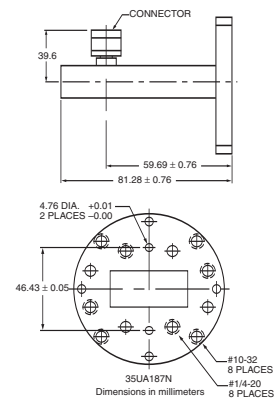
35UA187N outline
