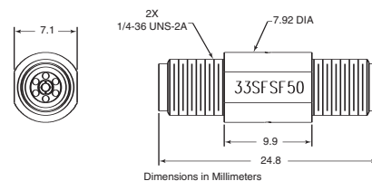
33SFSF50 outline
