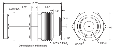
WI-102M, WI-105M W1 Male Sparkplug Connector, DC-110 GHz
