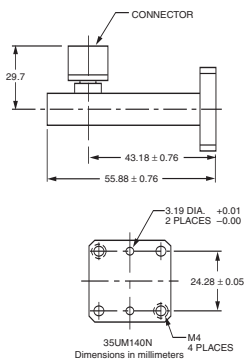
35UM140N outline
