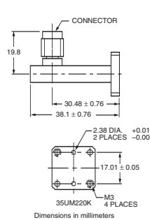
35UM220K outline
