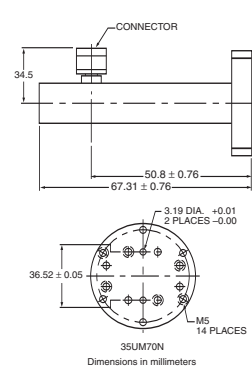
35UM70N outline
