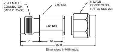
34VFK50 outline
