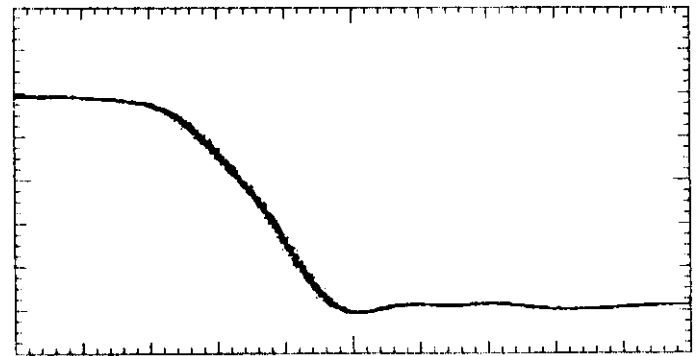
2 V/div and 50 ps/div Trailing edge 110 ps Falltime.
