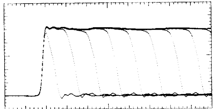
2 V/div and 200 ps/div Adjustable Duration from 100 ps to 10 ns in 2.5 ps steps.
