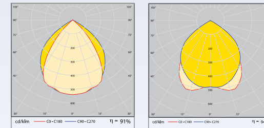
RANA D 1x28W FHE 1092 Mirror bright louvre
