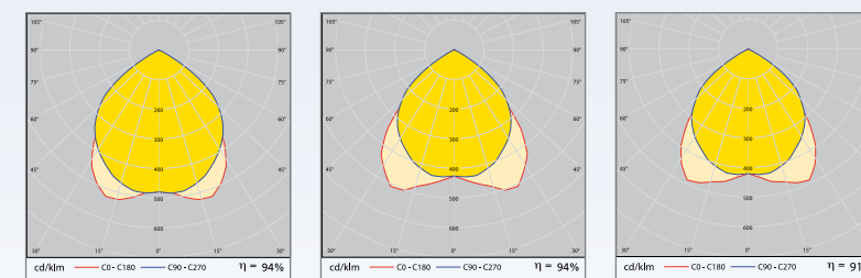
RANA 600 2x28W FHE 1092 Mirror bright louvre
