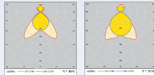
RANA D+I 1x28W FHE 1092 Mirror bright louvre
