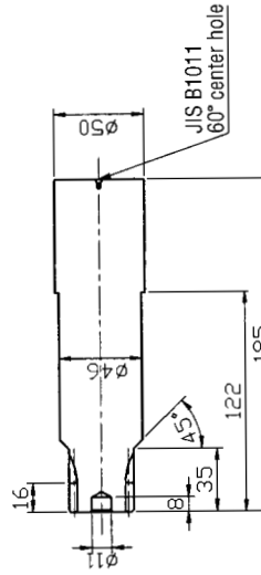
Detail of input gear (standard type B)
