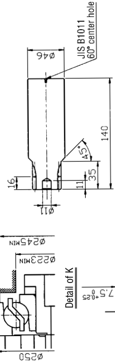
Detail of input gear (standard type A)
