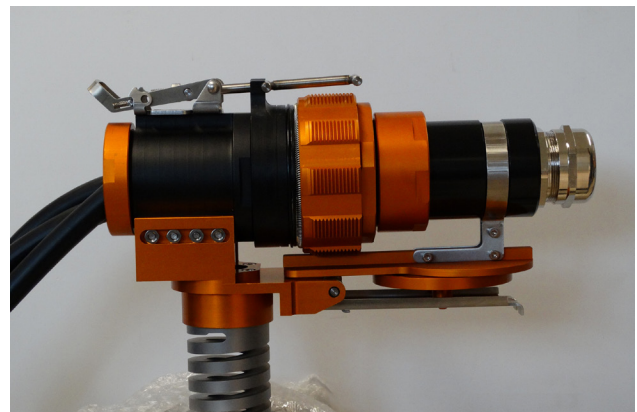
Glenair high-power tractor connector with TurboFlex™ cable, locking/lever coupling, and flexible standoff
