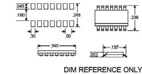
SO-14 Package
