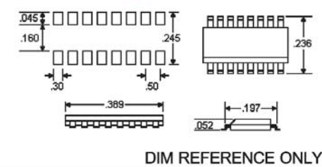
SO-16 Package
