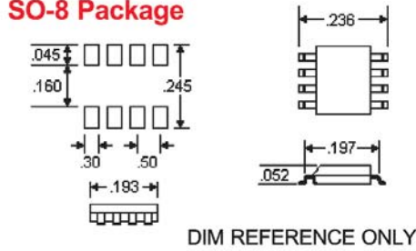
SO-8 Package
