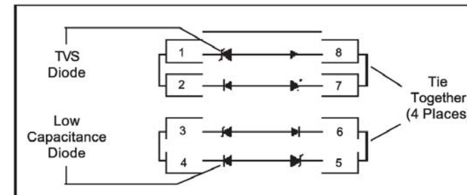
Figure 1. Electrical Configuration.
