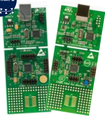
STM8S-DISCOVERY STM8SVLDiscovery
