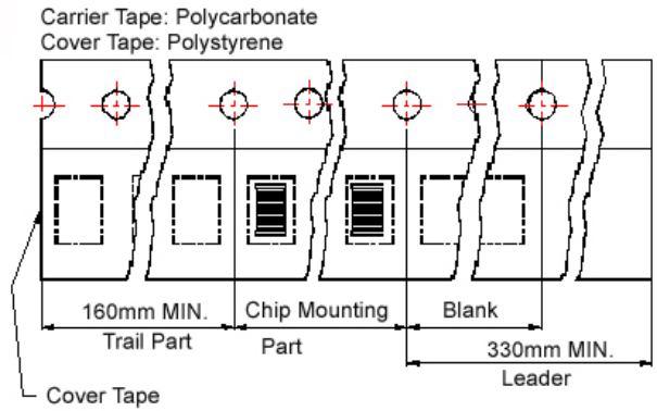
Tape Material
