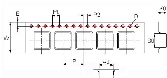
Tape Dimensions
