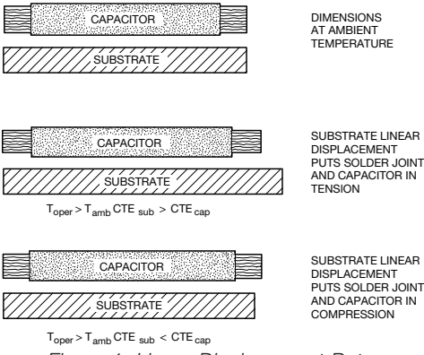
Figure 1. Linear Displacement Between Component and Substrate
