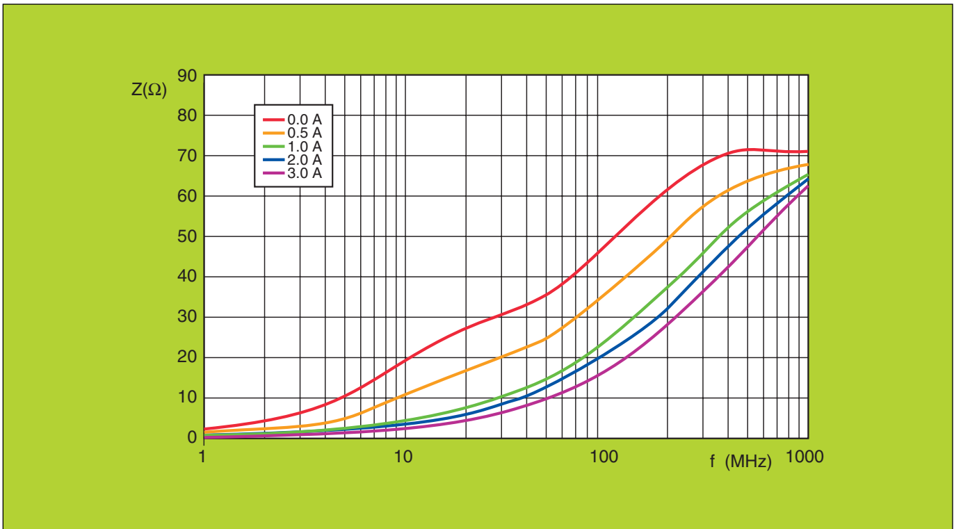
Fig. 10 Effect of bias current on the impedance of a 4S3 SMD bead. ( measured on BDS3/3/4.6 beads)
