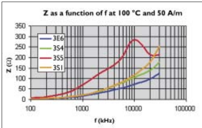
Fig. 3 Impedance curves at 100 °C, measured on a toroid Ø14 x Ø9 x 5 mm with 5 turns
