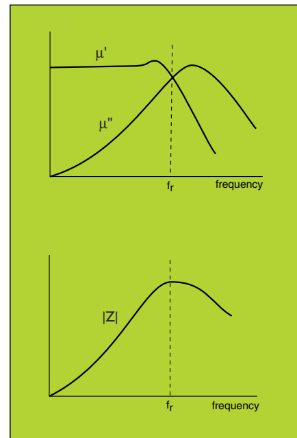
Fig. 14 Complex permeability and impedance.
