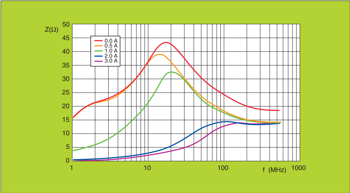
Fig. 7 Effect of bias current on the impedance of a 3S1 SMD bead. ( measured on BDS3/3/4.6 beads)
