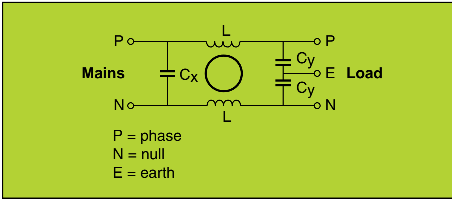
Fig. 12 Typical mains filter configuration.
