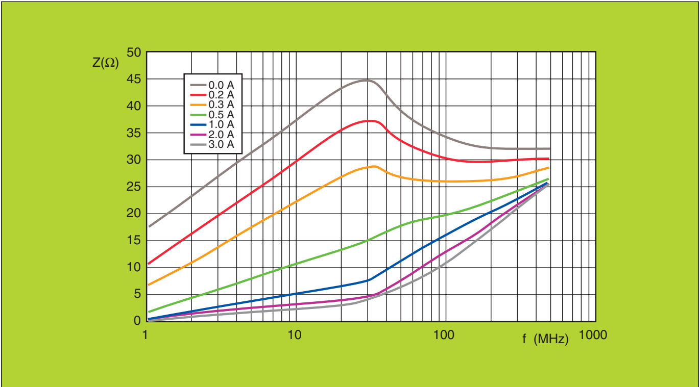
Fig. 8 Effect of bias current on the impedance of a 3S5 SMD bead. ( measured on BDS3/3/4.6 beads)
