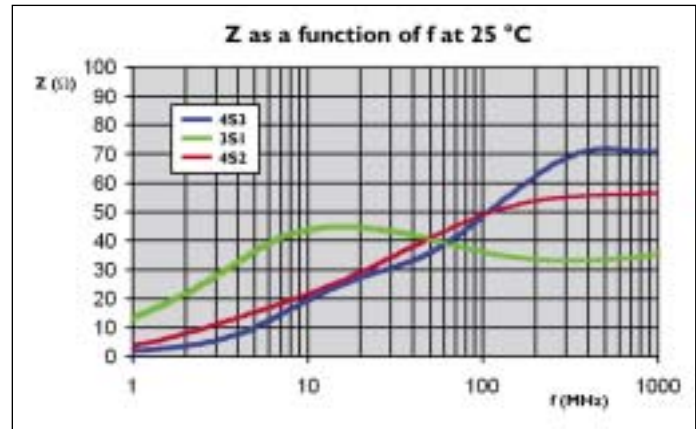
Fig. 4 Impedance curves at 25 °C, measured on an SMD bead 3 x 3 x 4.6 mm with 5 turns
