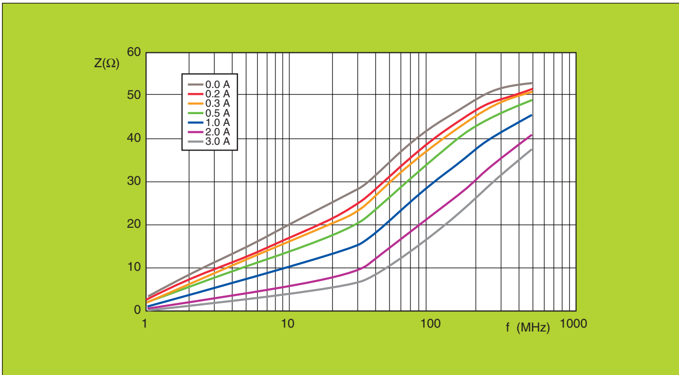
Fig. 9 Effect of bias current on the impedance of a 4S2 SMD bead. ( measured on BDS3/3/4.6 beads)
