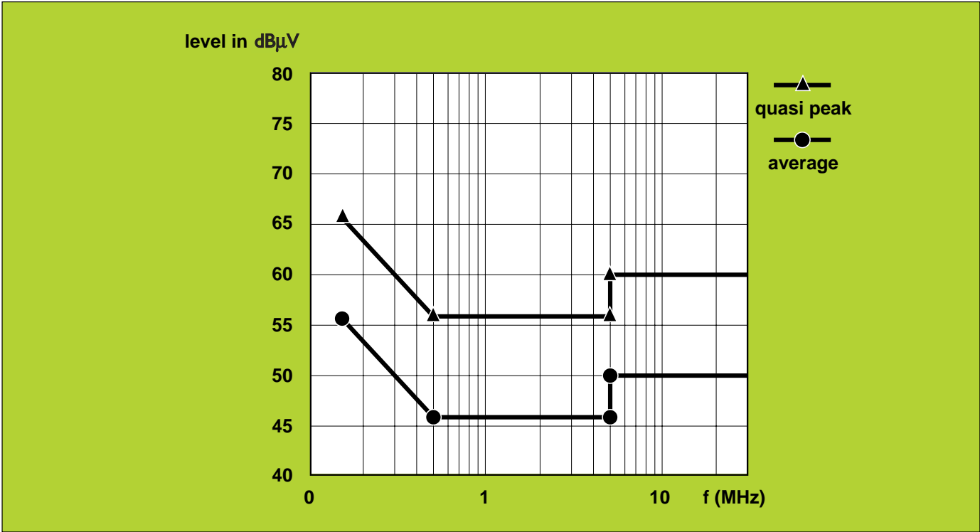
Fig. 1a European generic emission norm 61000-6-3 (residential, commercial, light industry).
