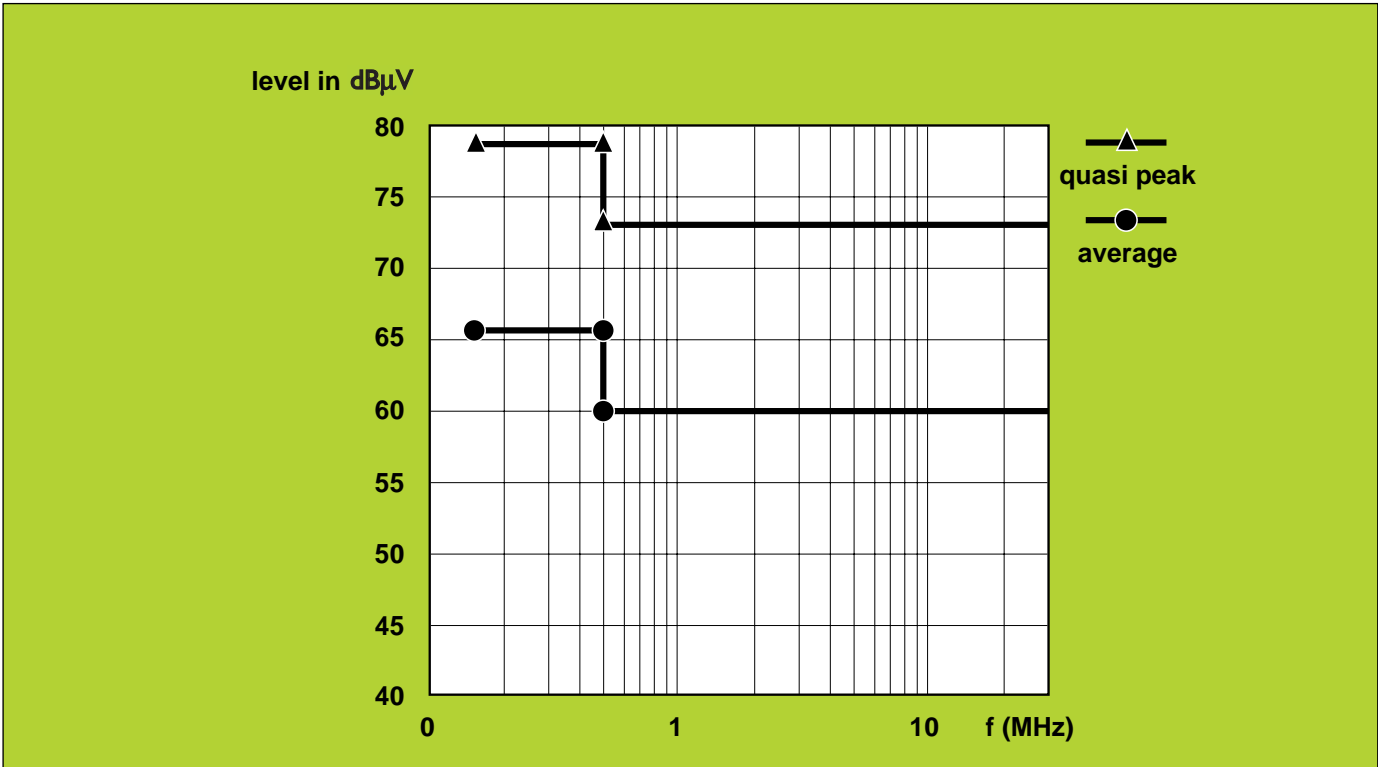
Fig. 1b European generic emission norm 61000-6-1 (industrial environment).
