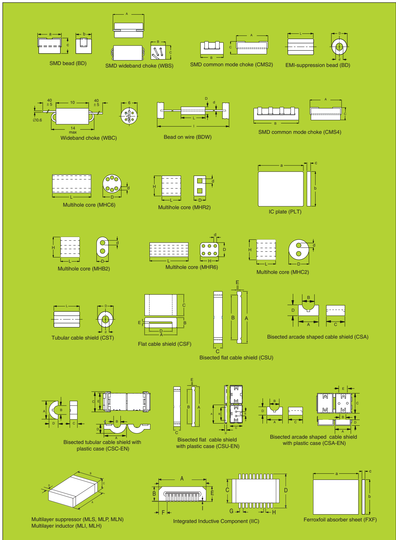
Fig. 11 Overview of small signal suppression products
