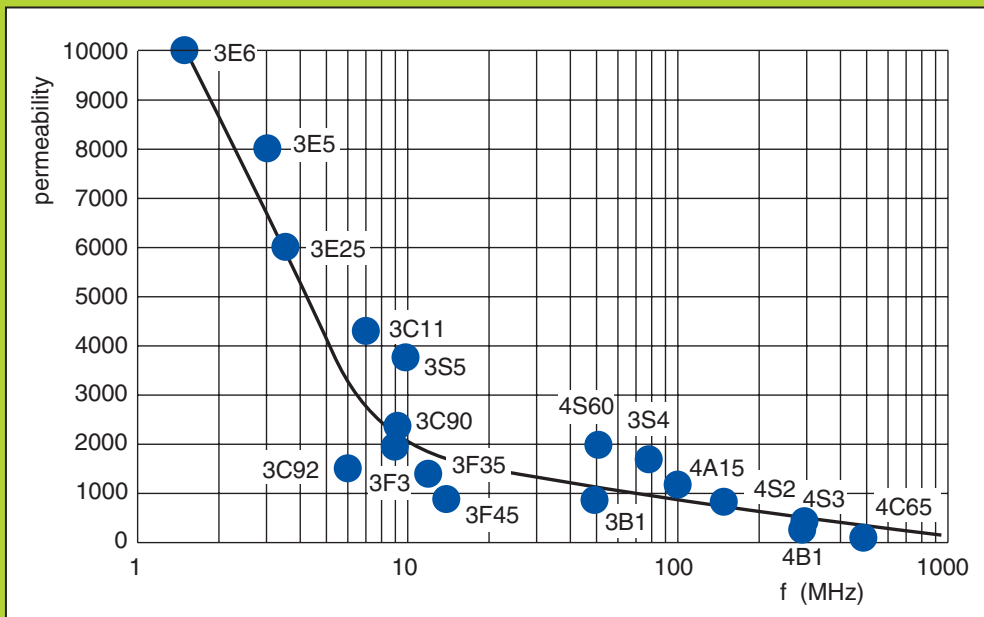
Fig. 6 Frequency of impedance peak for some ferrite materials.
