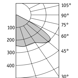
INSEL LB/R LED 100 D120
