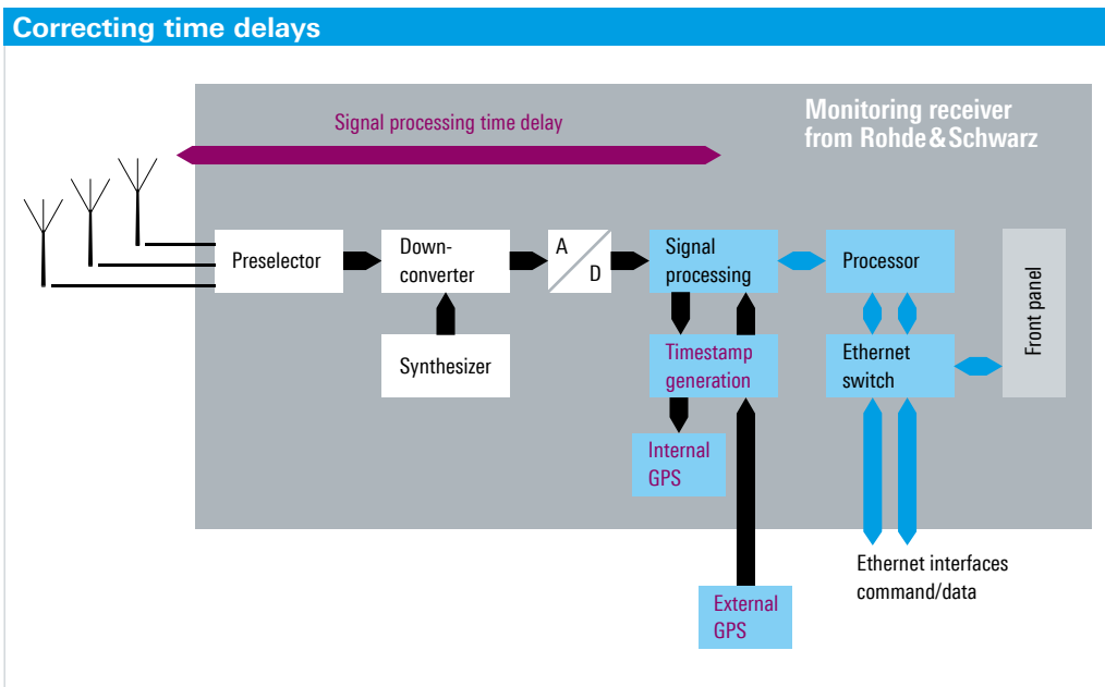
Rohde & Schwarz devices measure the time delay between antenna input and signal processing. This substantially boosts location accuracy.
