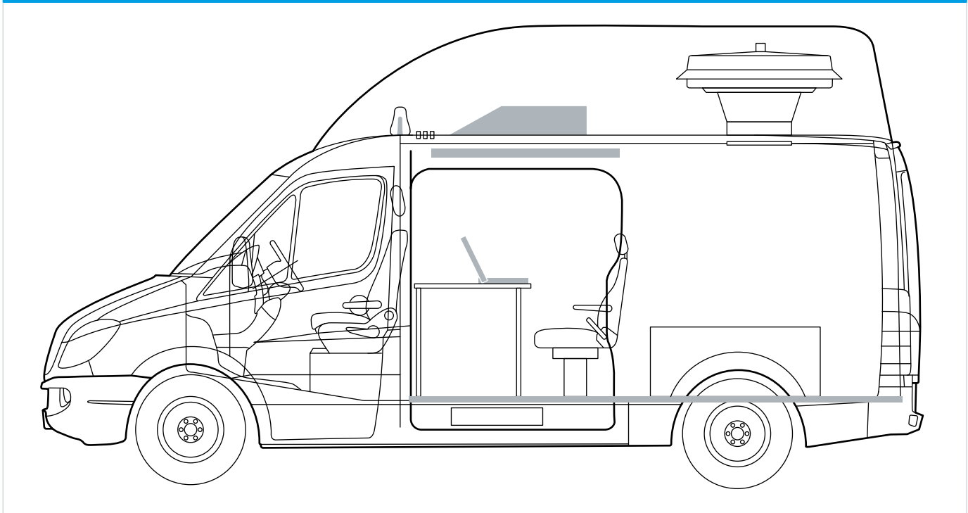
Surveillance system (not visible from outside)
