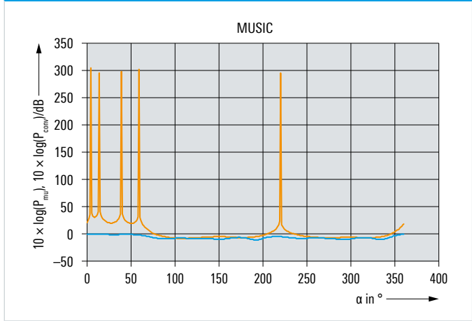
Fig. 28: DF function with MUSIC algorithm (S/N = 10)
