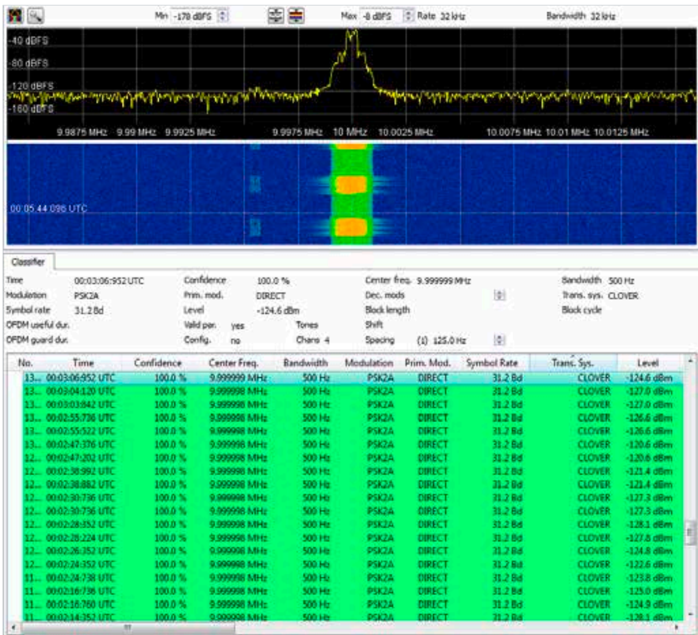
The classifier continuously measures technical signal parameters such as center frequency, bandwidth, symbol rate, modulation type and transmission system. It recognizes this signal as an HF CLOVER modem with the corresponding parameters.
