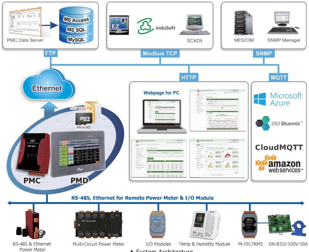
▲ System Architecture
