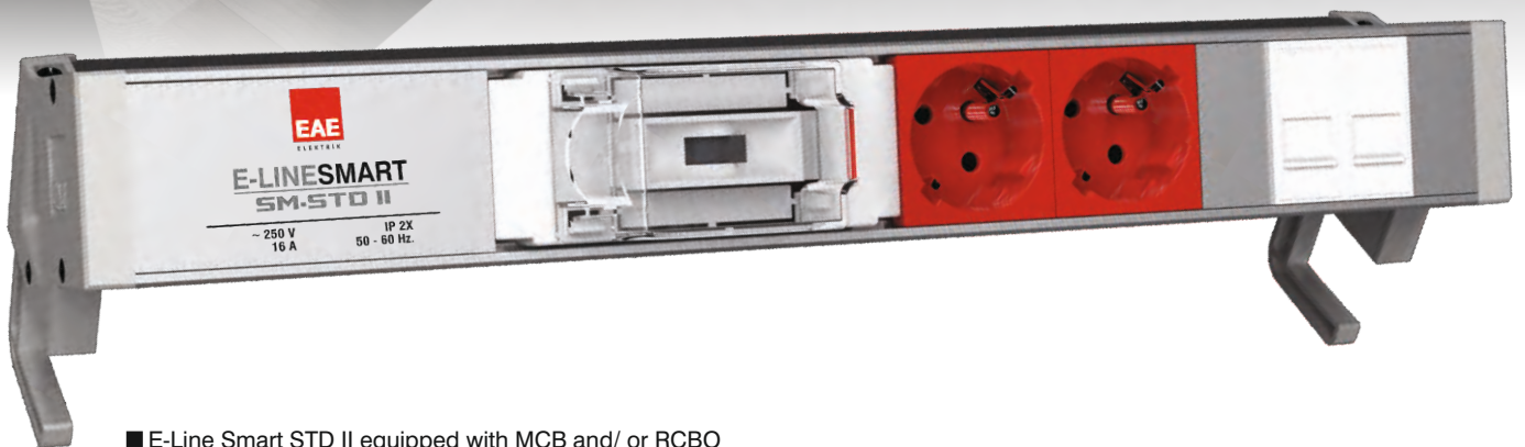
■ E-Line Smart STD II equipped with MCB and/ or RCBO
